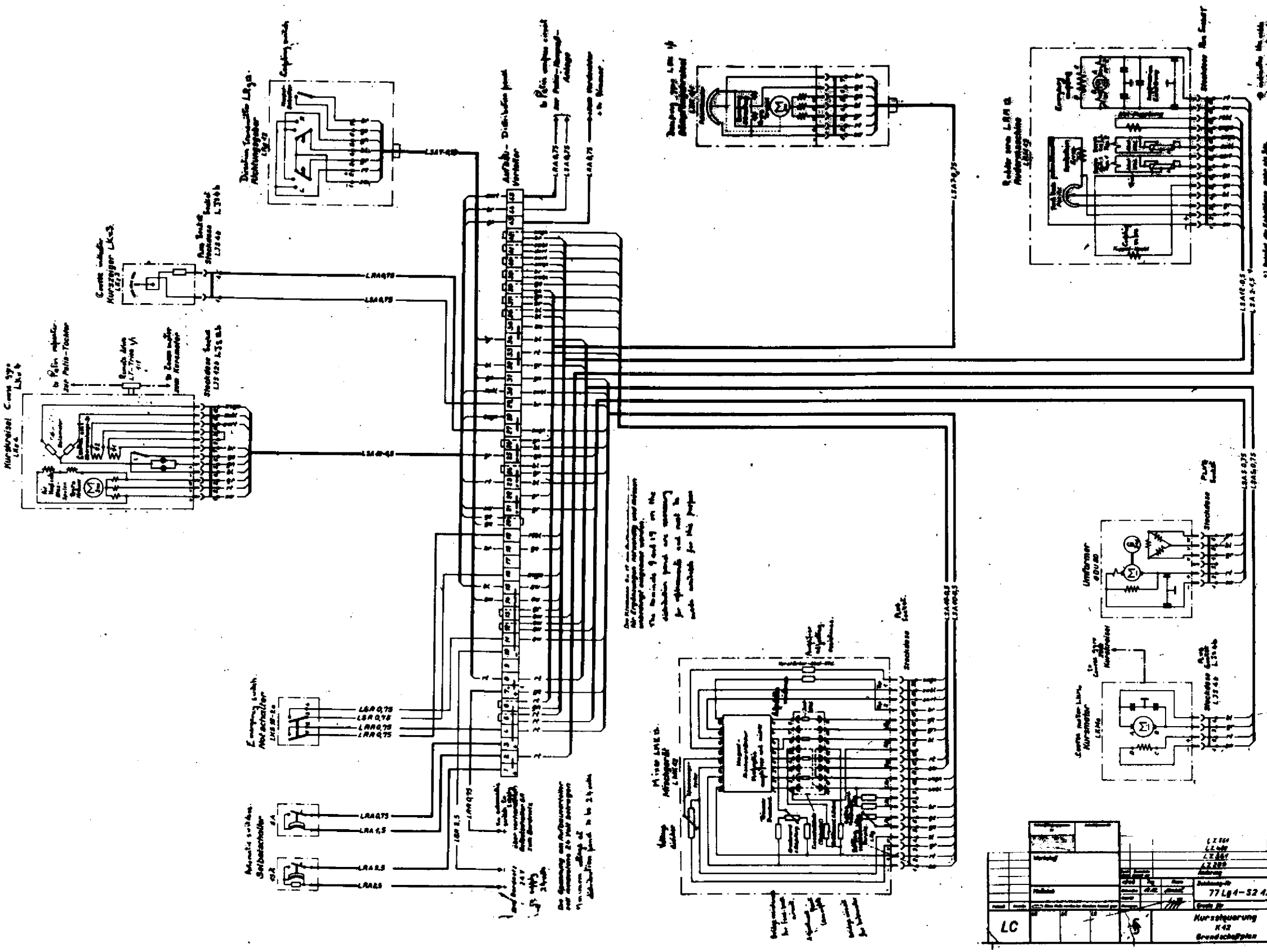
FIG. 4 CORE CONTROLLER K12 INSTALLATION WIRING DIAGRAM
