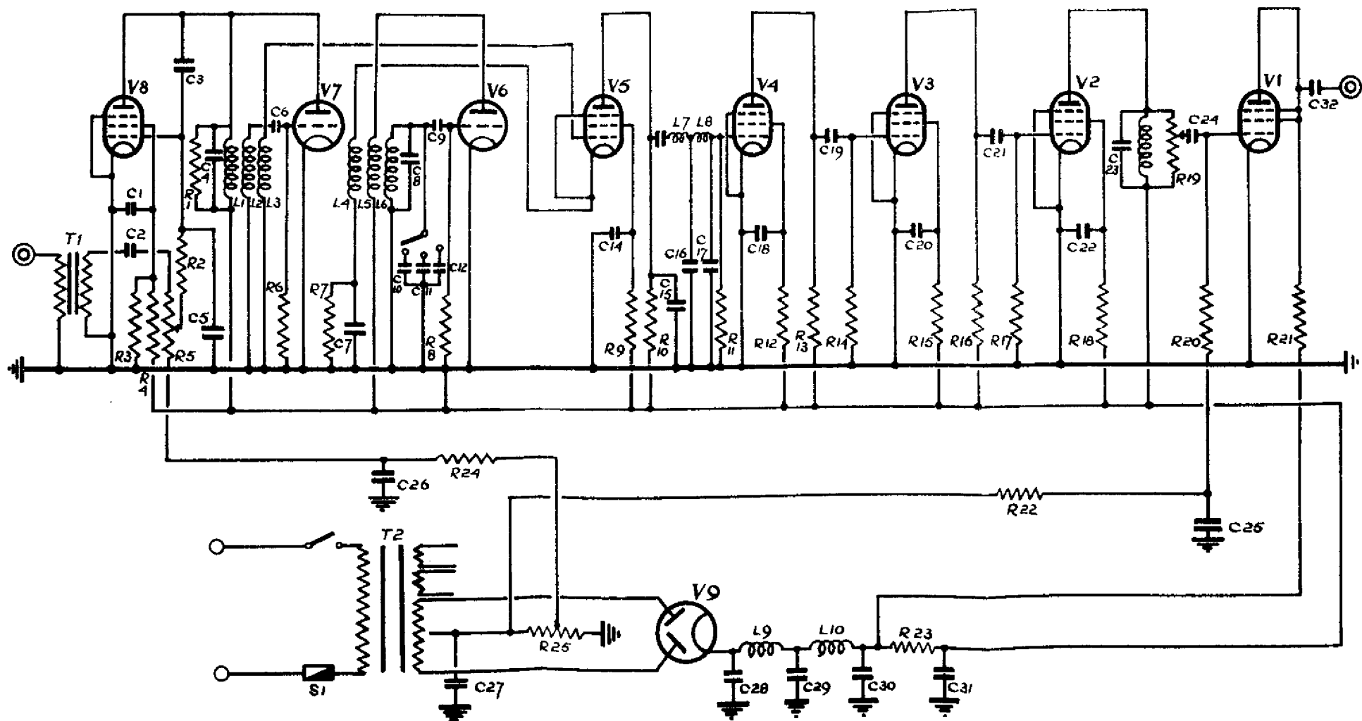
FIG. 139. MODULATOR & TRANSMITTER.
